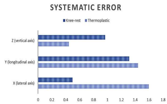
Fig. 1: Systematic error
